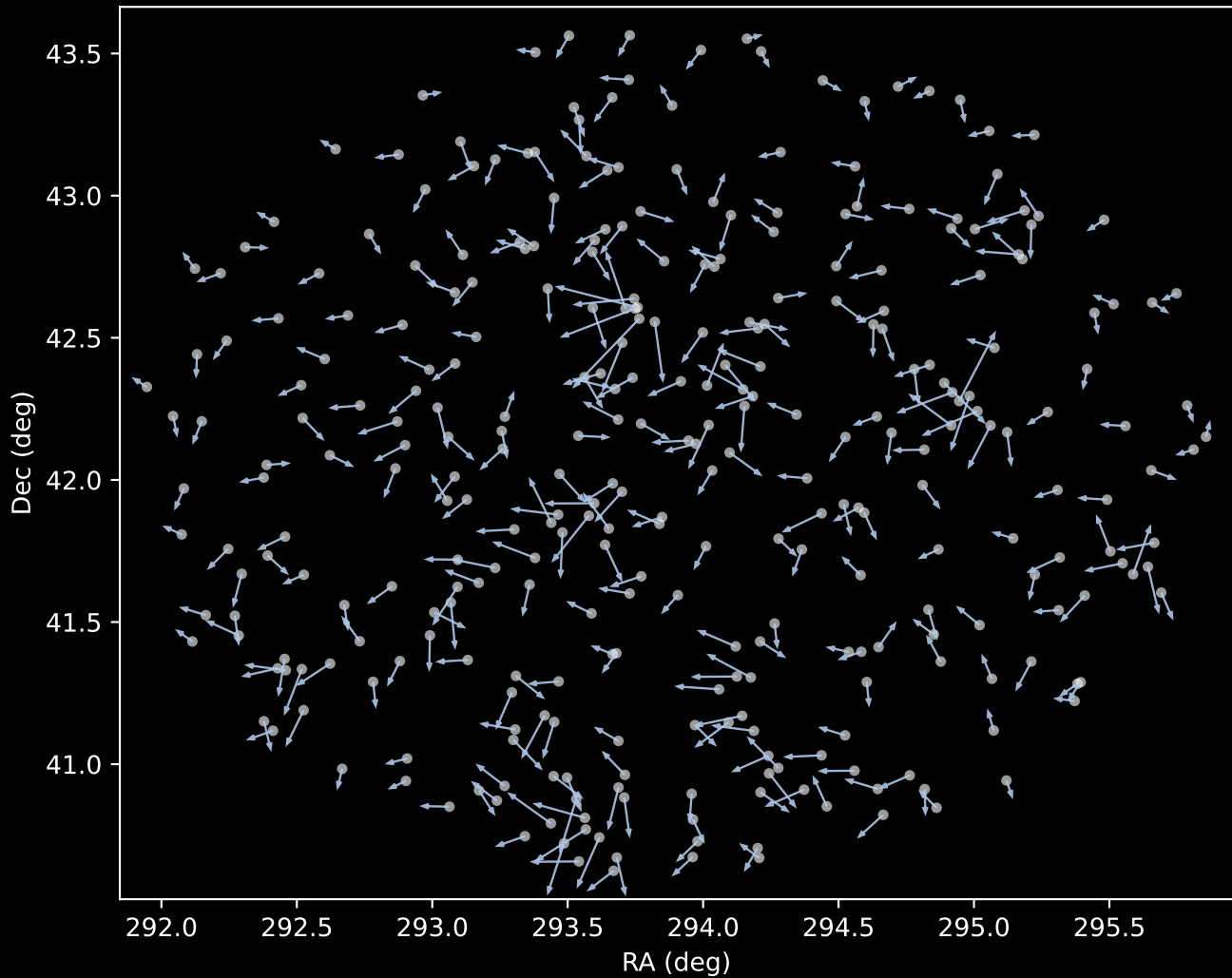
APOGEE DR17 Cluster 1 Proper Motion Vectors (n=322)
