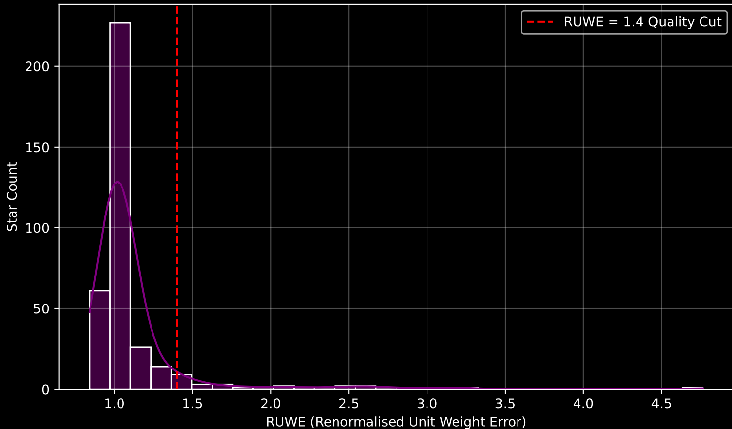
GAPOGEE DR17 Field [120+75] RUWE Distribution (n= 358)
