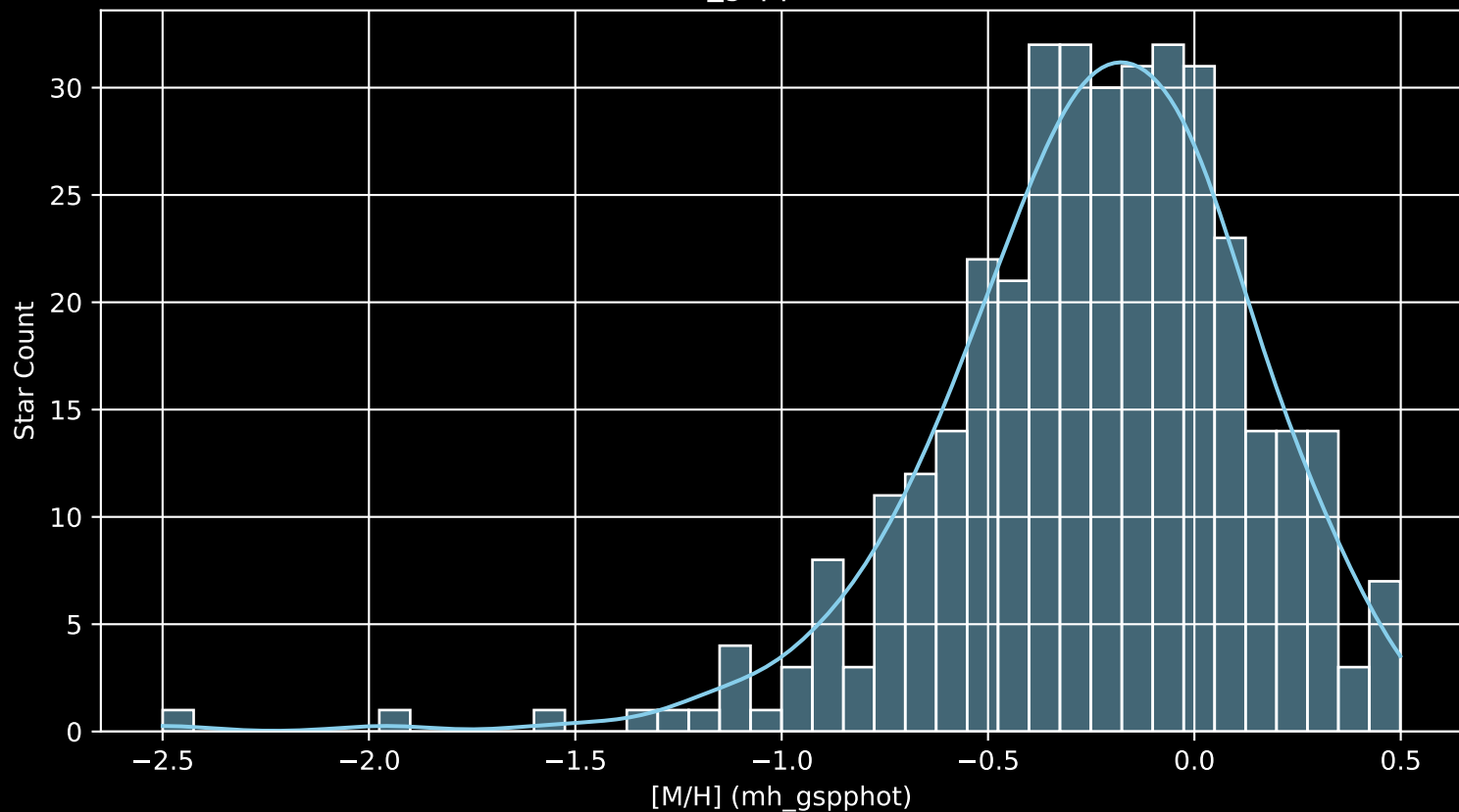
APOGEE DR17 Field: [120+75 [M/H] (mh_gspphot) (n= 368)
