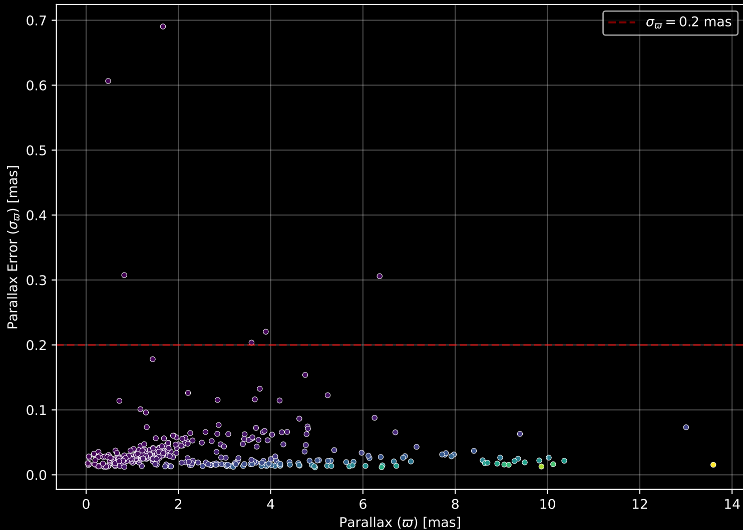
APOGEE DR17 Field: [120+75] Parallax Quality (n= 372)
