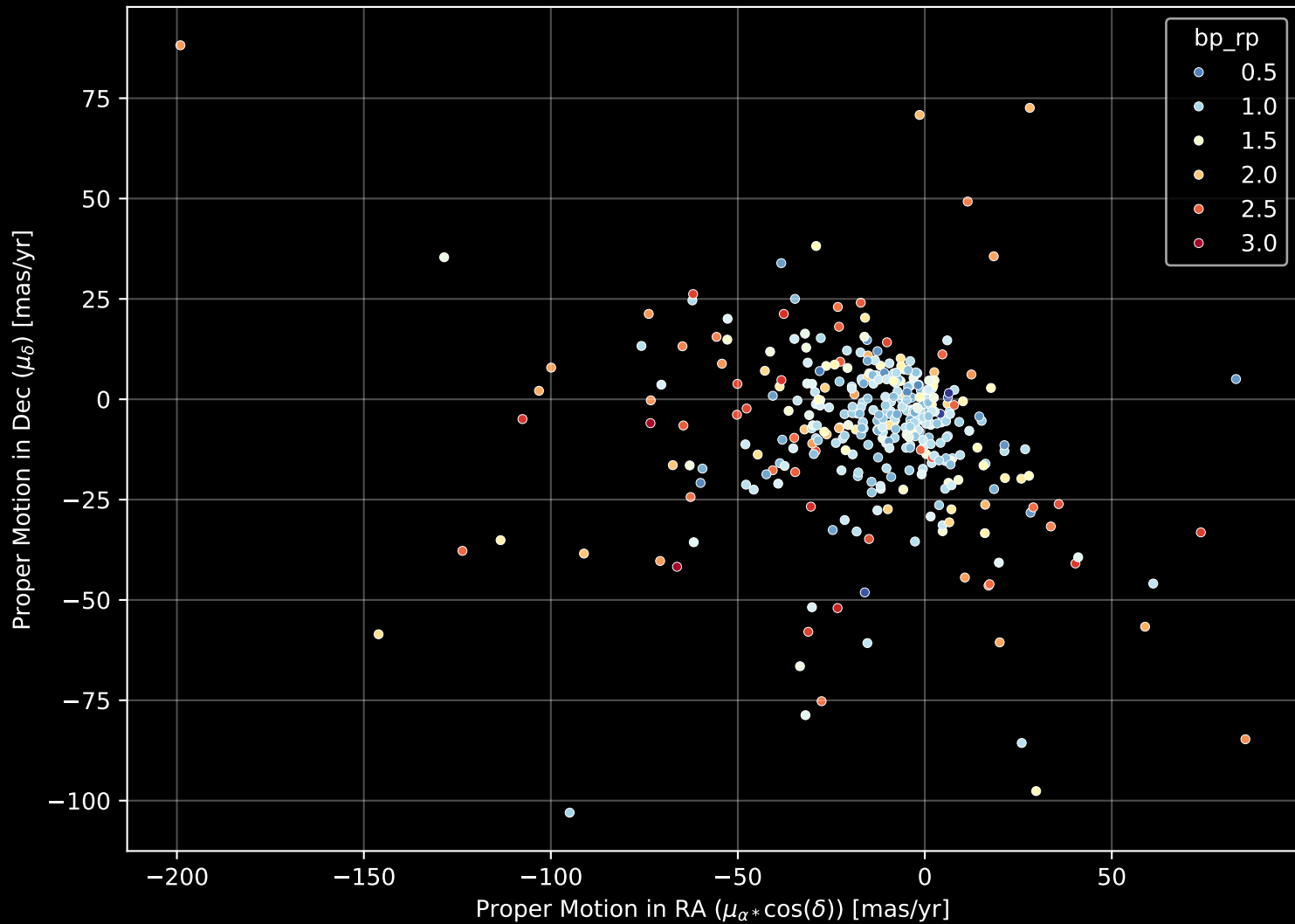
APOGEE DR17 Field: [120+75] Proper Motion Diagram (n= 372)
